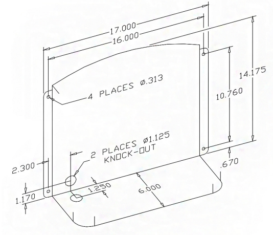
Figure 6. CS-100 Installation Template
