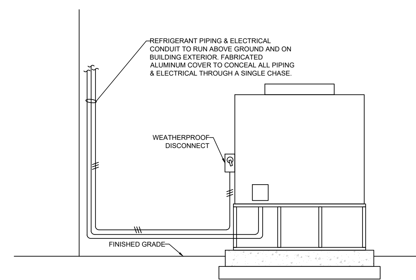
4 OUTDOOR UNIT SCHEMATIC E-1 SCALE: NTS
