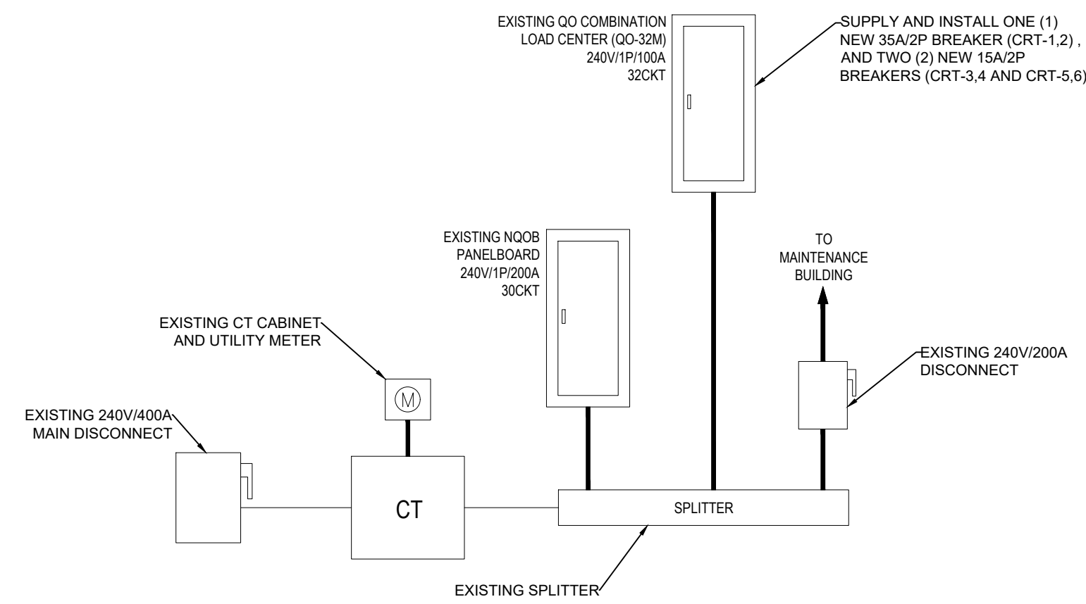
3 ELECTRICAL SCHEMATIC E-1 SCALE: NTS
