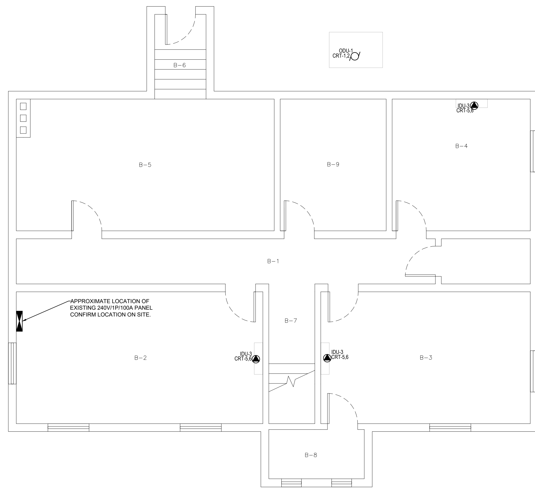
2 BASEMENT FLOOR PLAN E-1 SCALE: 1:50
